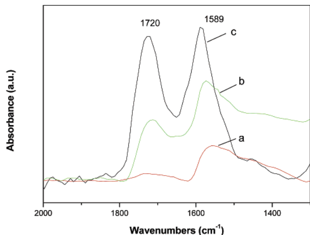
Figure 8. FTIR spectra of the SWNTs treated with different oxidation process: (a) gas-phase oxidation, (b) refluxing in 2.6 M \text{HNO}_3 , and (c) sonication in \text{H}_2\text{SO}_4/\text{H}_2\text{O}_2 .
