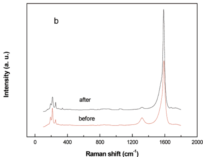
Figure 6. SEM image of the location of TiO 2 nanoparticles on gas-phase oxidation SWNTs (a; inset shows a magnified view) and the Raman spectra of SWNTs before and after gas-phase oxidation in air at 500 °C for 1 h (b).
