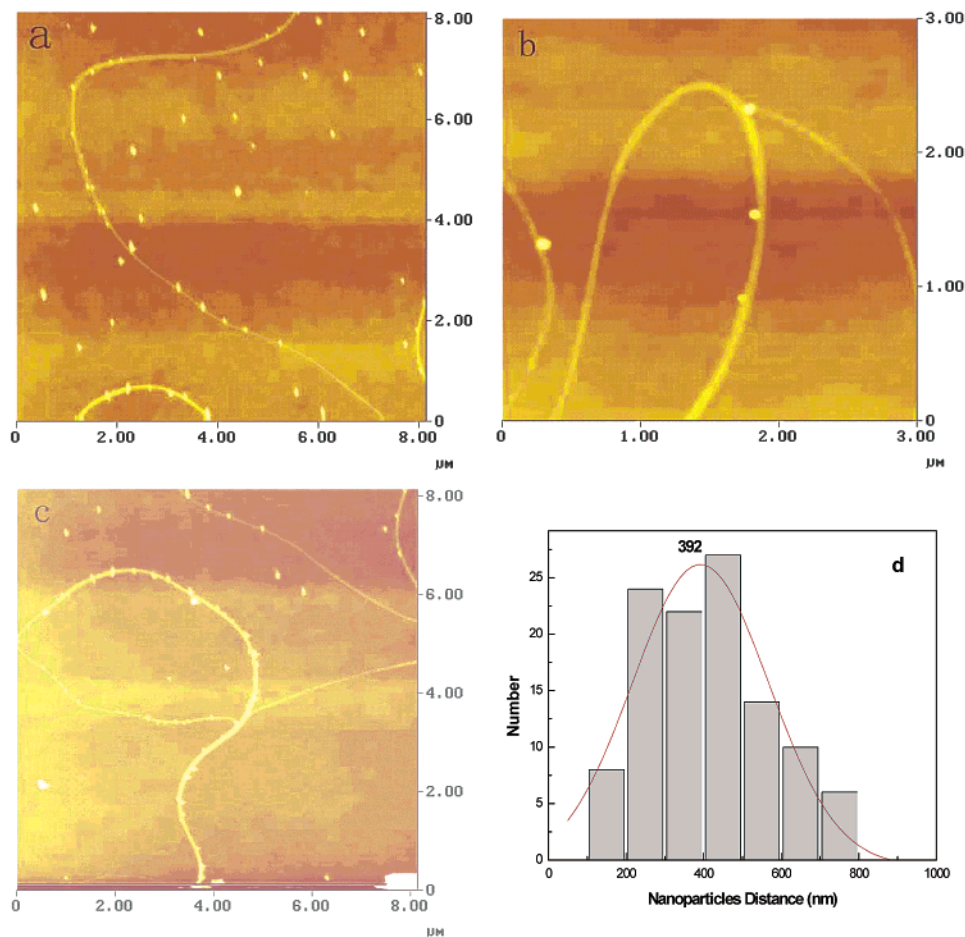
Figure 4. AFM images of the location of TiO 2 nanoparticles on SWNTs after refluxing in 2.6 M HNO 3 (a), of a magnified view (b), of the location of TiO 2 nanoparticles on the thicker bundles of SWNTs (c), and the corresponding histogram of the TiO 2 nanoparticle distances (d). The solid lines correspond to Gaussian fits.
